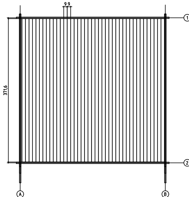
FLOOR BOARDS - FUSSBODENBRETTER - PLAN POSE PLANCHER
