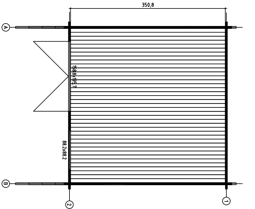
FLOOR BOARDS - FUSSBODENBRETTER - PLAN POSE PLANCHER
